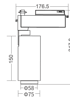
3-pin track adaptor
