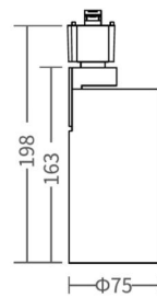
3-pin track adaptor
