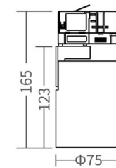
4-pin track adaptor
