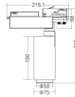
4-pin track adaptor
