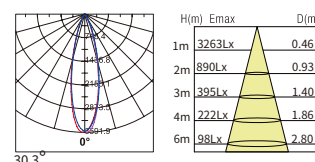
30° 15W
