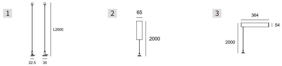
1 MP-KIT-SUS01 suspended kit for surface track 200CM CABLE 2 MP-KIT-SUS02 suspended kit with driver box for surface track 3 MP-KIT-SUS03 suspended kit with driver box for surface track
