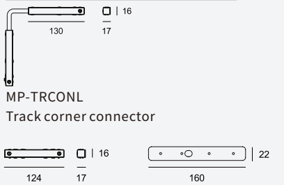
MP-TRCONL Track corner connector MP-TRCON Track connector
