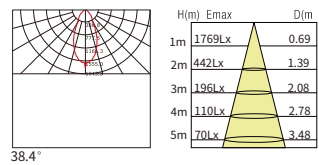
30° 15W
