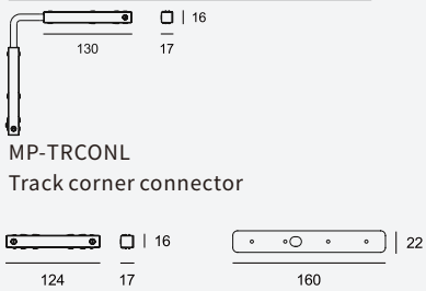
MP-TRCONL Track corner connector MP-TRCON Track connector
