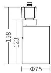
3-pin track adaptor
