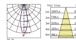
30° 10W
