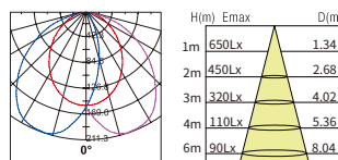
diffuser 20W
