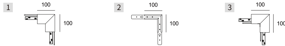
1 MP-SUR-VER90 vertical track corner 90° surface+circuit corner connector 2 MP-SUR-HOR90 horizontal track corner 90° surface+circuit corner connector 3 MP-SUR-EXT90 external track corner 90° surface+circuit corner connector
