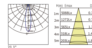
15° 10W
