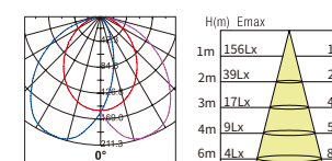
diffuser 10W
