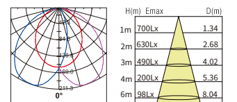
diffuser 30W
