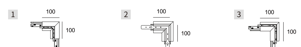
1 MP-RETR-VER90 vertical track corner 90° trimless+circuit corner connector 2 MP-RETR-HOR90 horizontal track corner 90° trimless+circuit corner connector 3 MP-RETR-EXT90 external track corner 90° trimless+circuit corner connector
